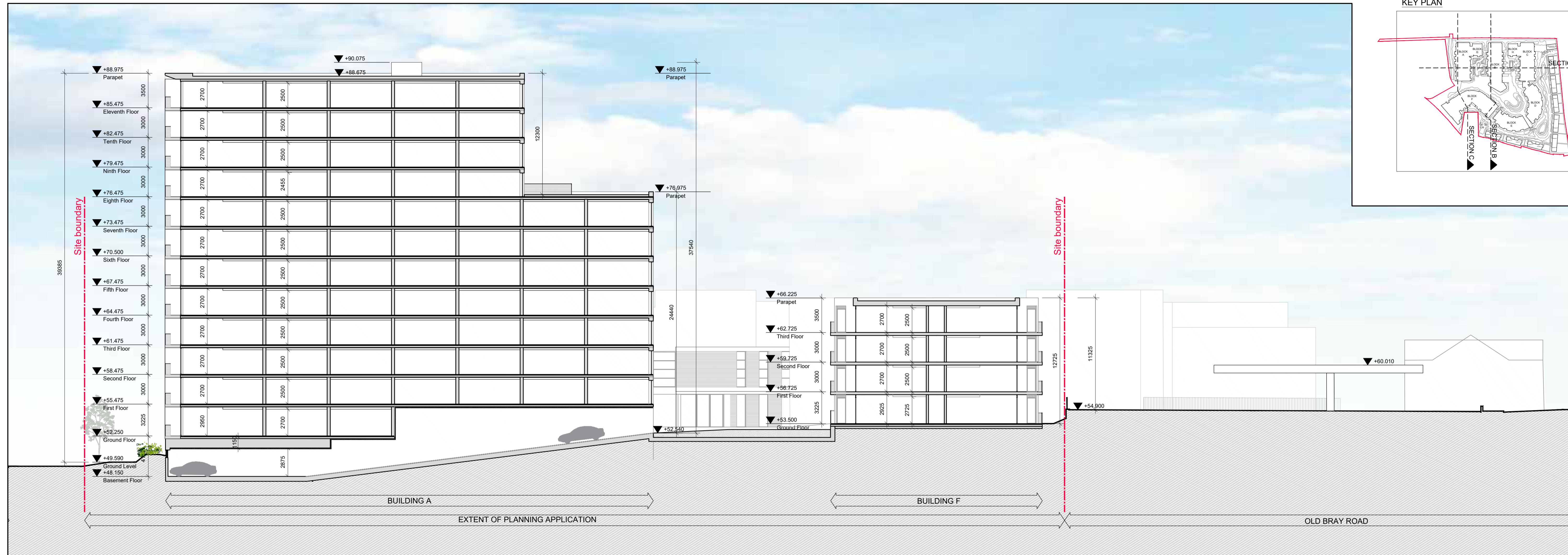
01 PROPOSED SECTION C PL3002 SCALE 1:200
